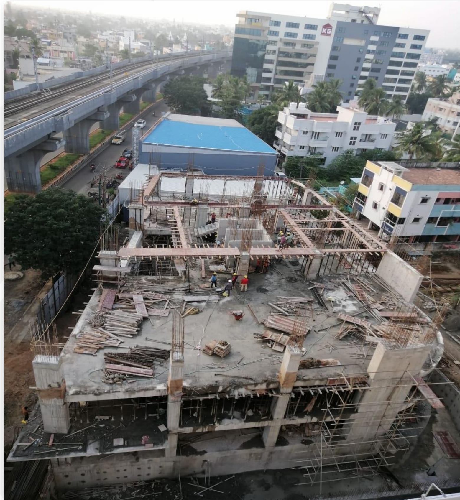
Second Floor Column Concreting Work Completed
