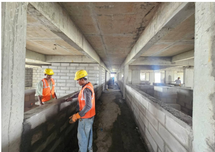
Second Floor P1 - Roof Slab Shuttering
