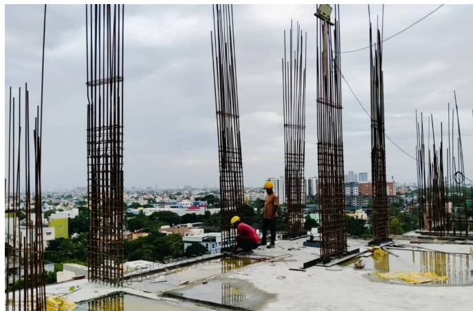
Tenth Floor P2 - Col Marking & Reinforcement
