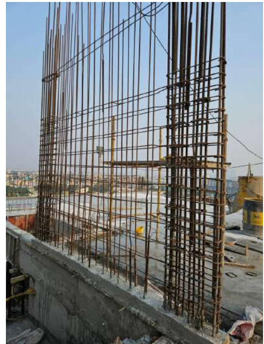
SHR - Col Marking & Reinforcement
