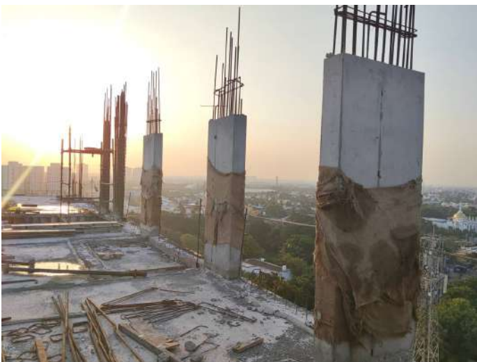
Twelfth Floor P1 - Column Concrete
