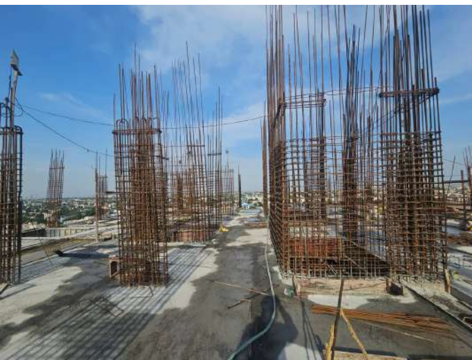
Twelfth Floor P1 - Col Marking & Reinforcement
