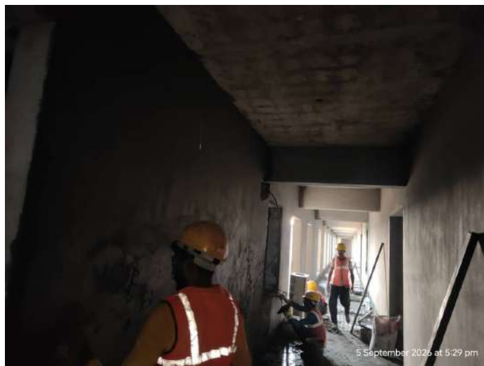
5F - Internal Plastering Corridor Area
