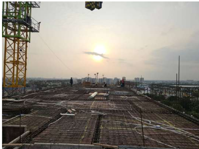
Twelfth Floor P1 - Slab & Beam Reinforcement
