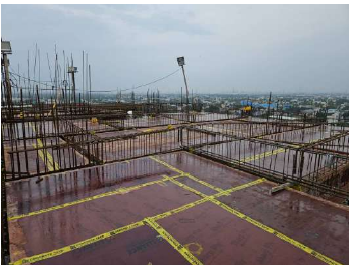
Twelfth Floor P2 - Slab & Beam Reinforcement
