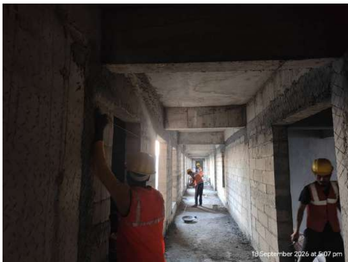
6F - Internal Plastering Corridor Area
