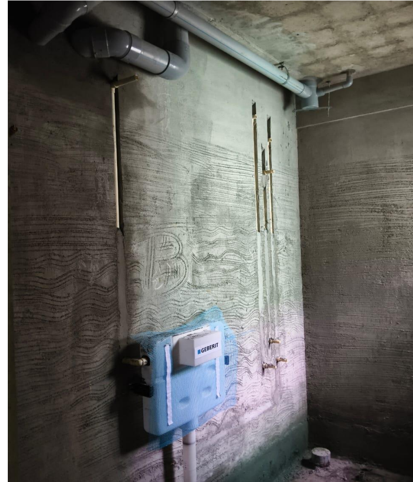
Block-3 Fourth Floor Suspended Pipeline Work in Progress
