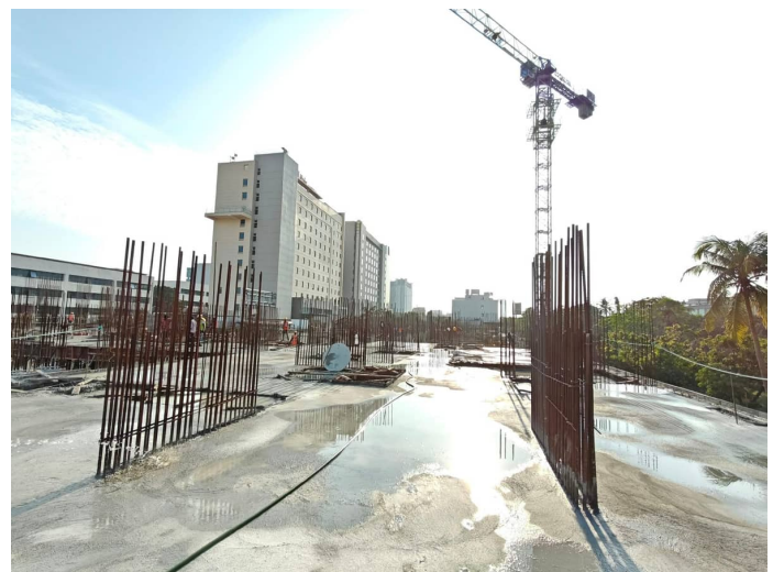
First Floor Slab Shuttering
