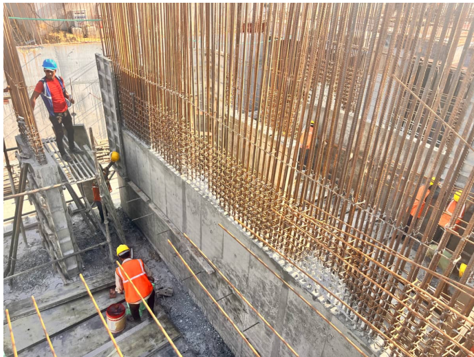
Retaining Wall & Column Shuttering
