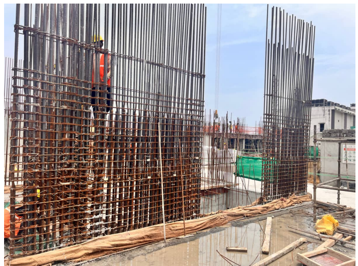
Column Reinforcement
