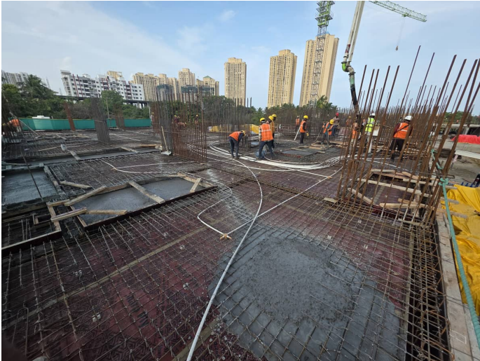
First Floor Slab Concrete
