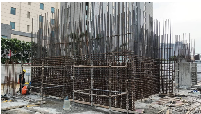
Column Reinforcement
