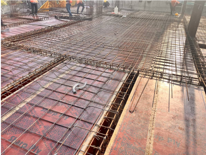
First Floor Slab Reinforcement
