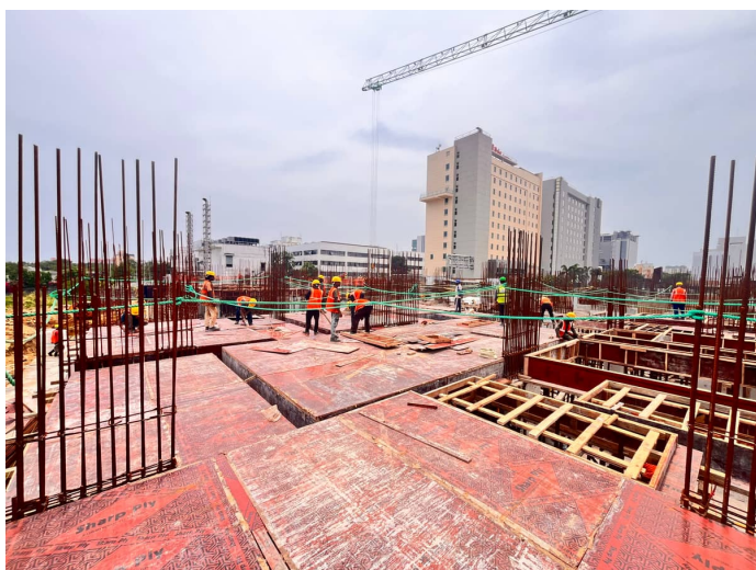
First Floor Slab Shuttering
