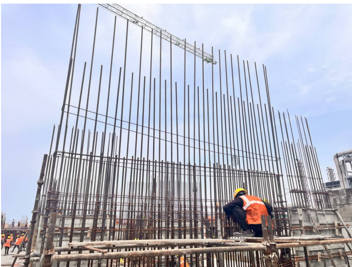
Column Reinforcement
