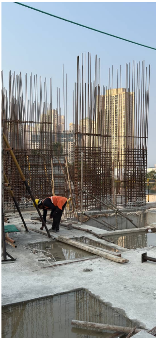
Column Reinforcement
