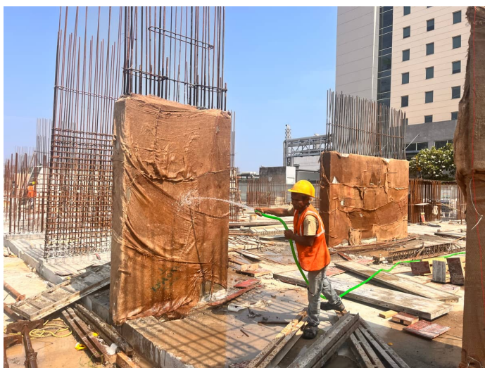
Column Concrete
