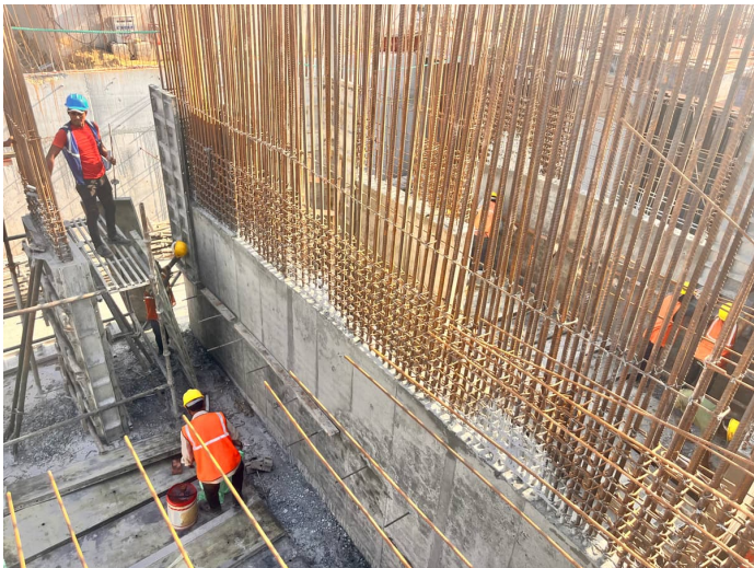
Retaining Wall & Column Reinforcement
