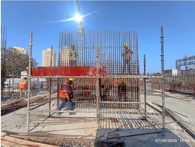
Column Reinforcement
