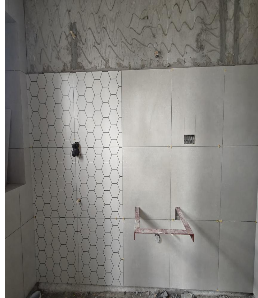
Villa No 5 – SFbedroomtoilet wall tilelaying work in progress
