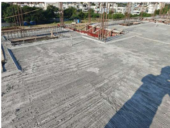
V89 - Completion of Staircase Headroom & Part Roof Slab
