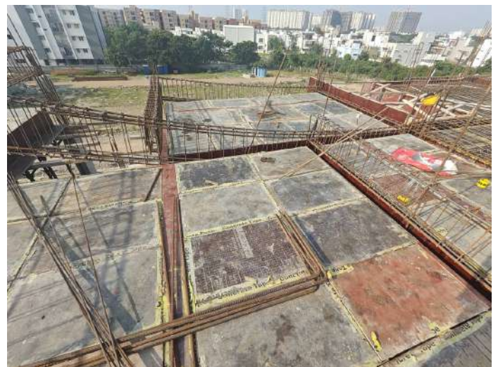
V93 - Stair Head Room Roof Slab & Beam - Shuttering, Reinforcement
