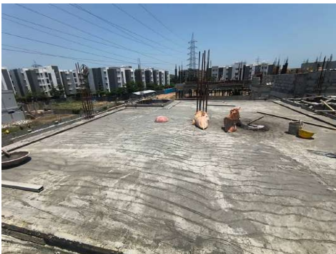
V62 - First Floor Roof Slab & Beam Concreting
