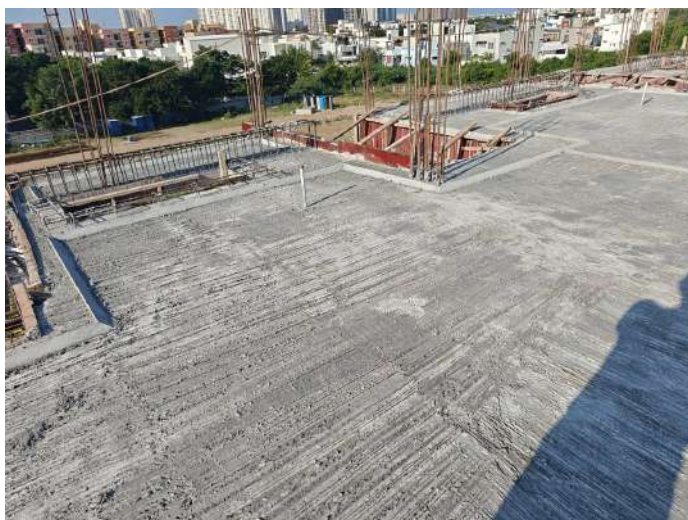
V89 - Stair Head Room Roof Slab & Beam Concreting
