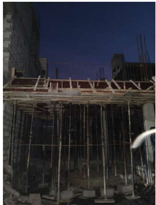
V34 - Ground Floor Roof Slab & Beam - Shuttering, Reinforcement
