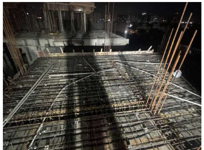
V103 - SF- Roof Slab & Beam - Shuttering, Reinforcement
