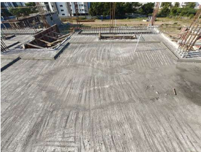
V93 - Stair Head Room Roof Slab & Beam Concreting
