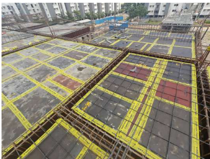
V87 - Stair Head Room Roof Slab & Beam - Shuttering, Reinforcement
