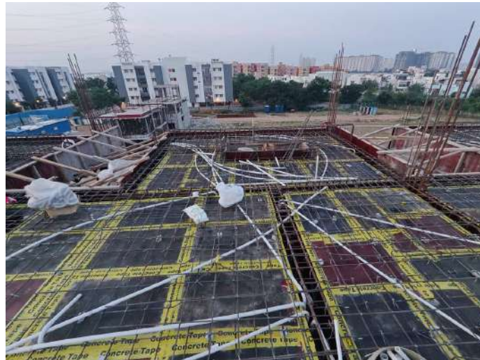
V90 - Stair Head Room Roof Slab & Beam - Electrical works
