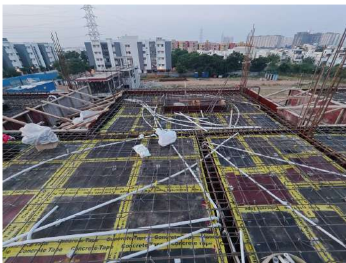
V90 - Stair Head Room Roof Slab & Beam - Shuttering, Reinforcement
