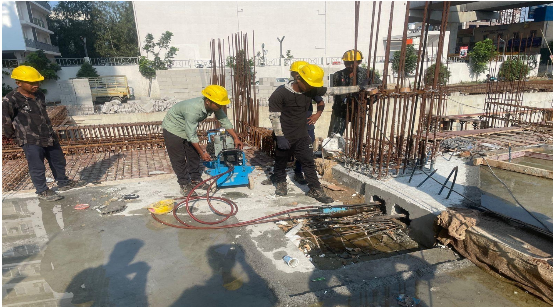
Tower -2 Commercial basement roof Tendon stressing work completed.
