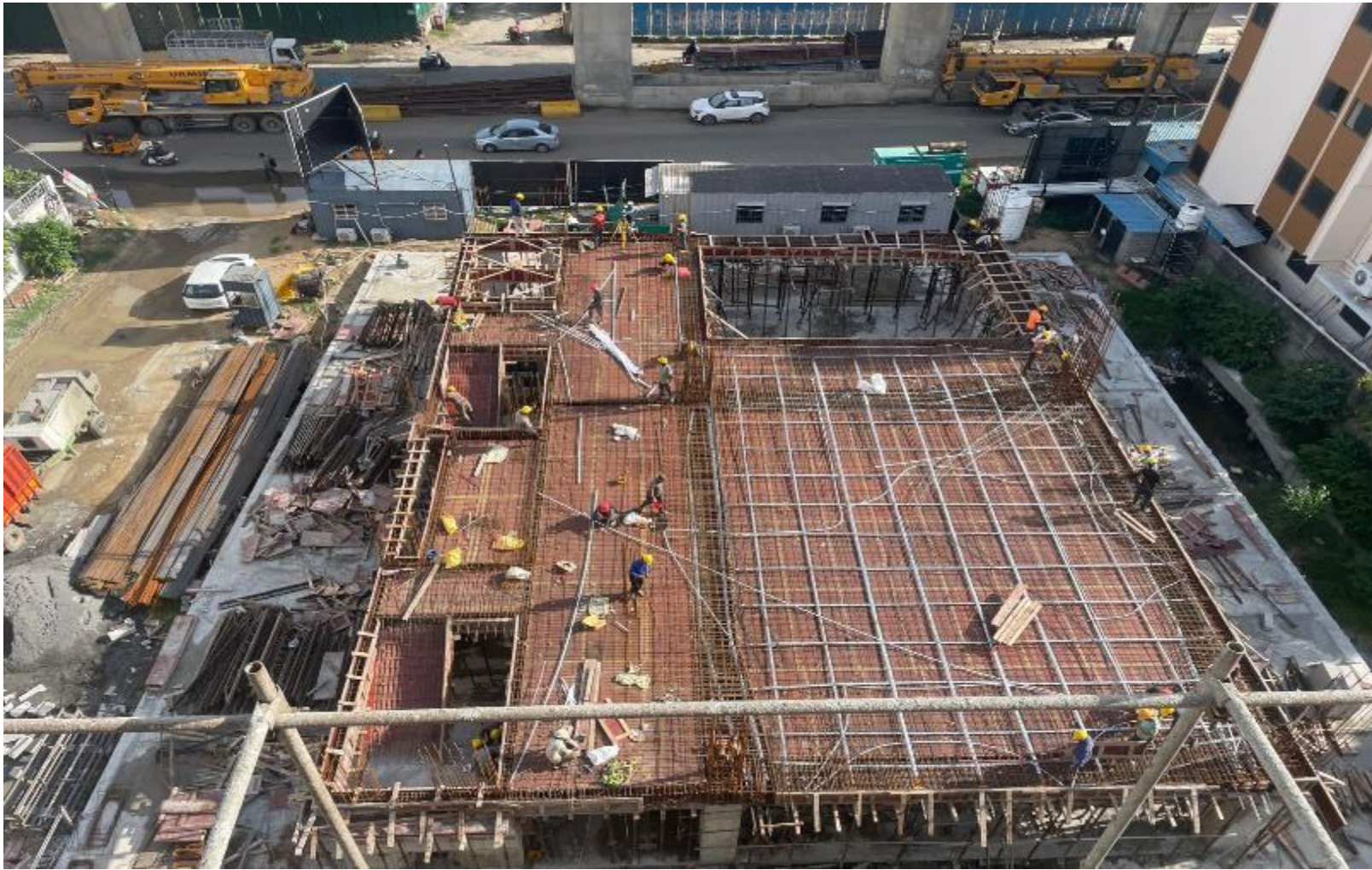
Tower -2 stilt floor roof reinforcement & PT works completed .
