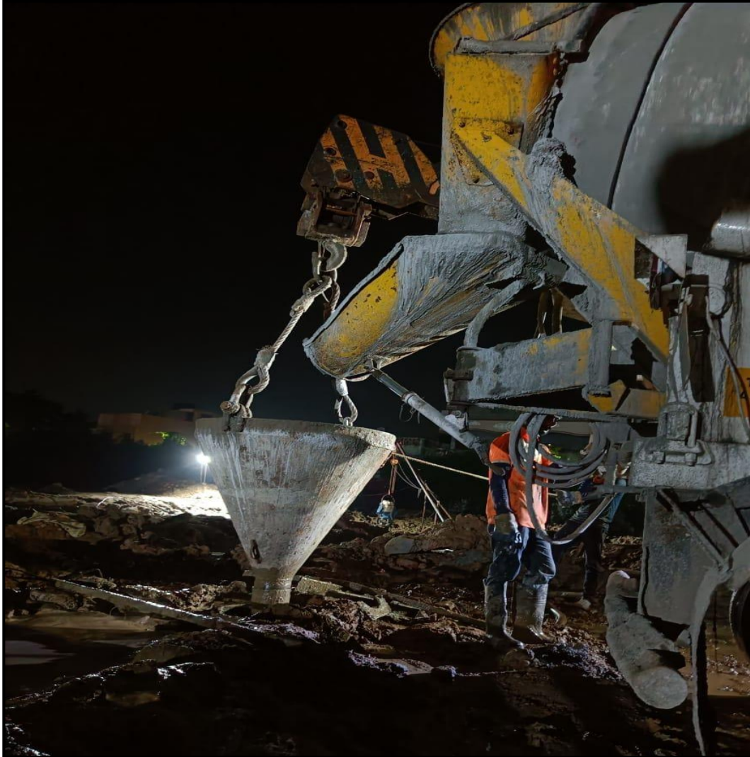
DRA Polaris - Piling concrete work in progress - 169/182 Nos completed
