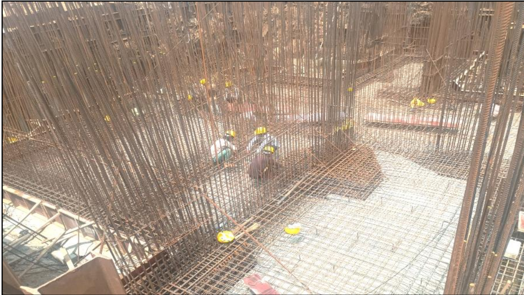
UG Sump – Raft & pile cap reinforcement & shuttering work completed
