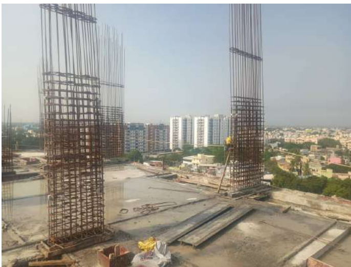
Reinforcement-Column
