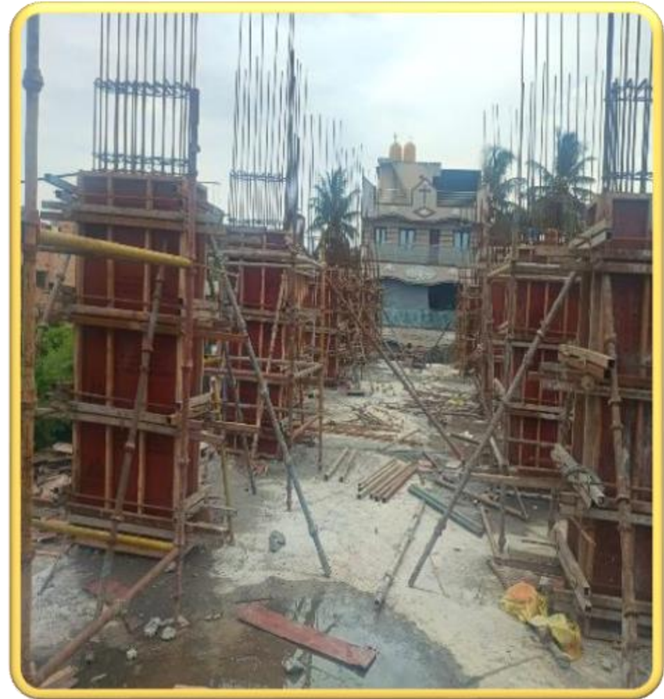
Main building – First Floor Pour 1 column Shuttering work
