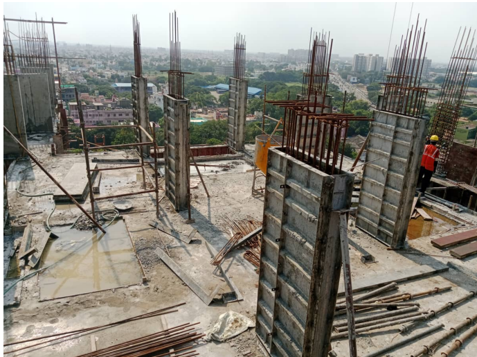
Thirteenth Floor P2 - Column Shuttering
