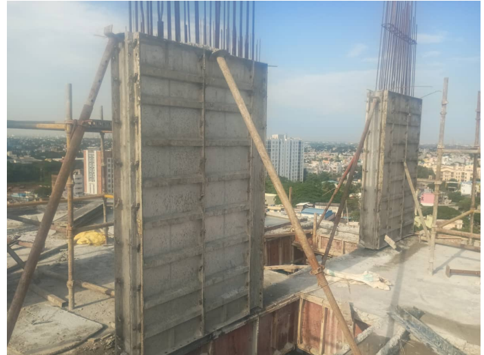
Thirteenth Floor P2 - Column Concrete
