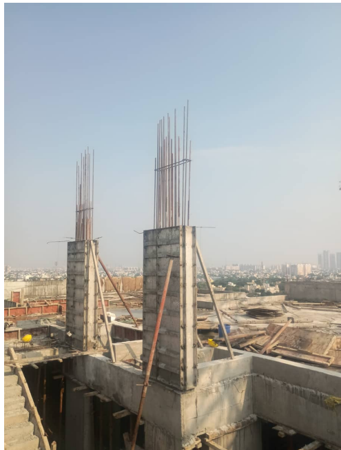
SHR - Column Shuttering
