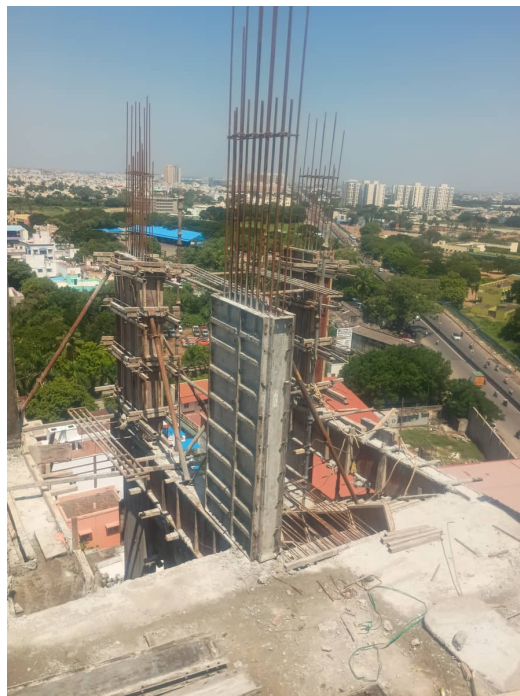
Thirteenth Floor P2 - Column Shuttering
