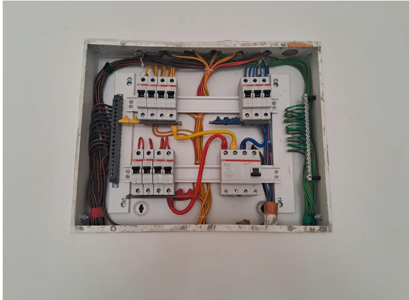
Wing 3D, 4 th Floor – Wiring Works in Progress
